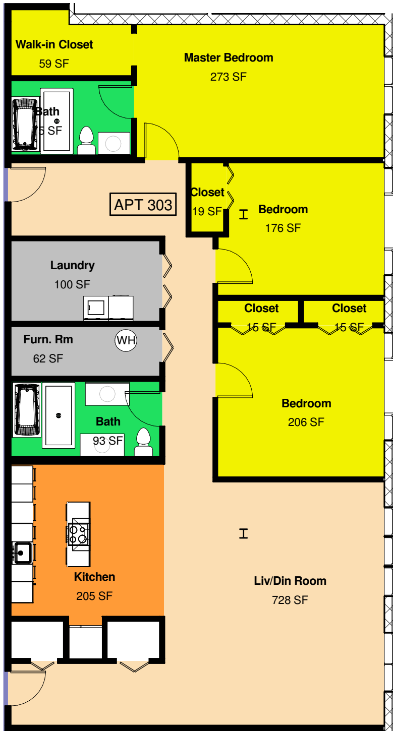
① Enlarged Proposed 3rd Floor Apt 303 - 2103 SF 1/8" = 1'-0"
