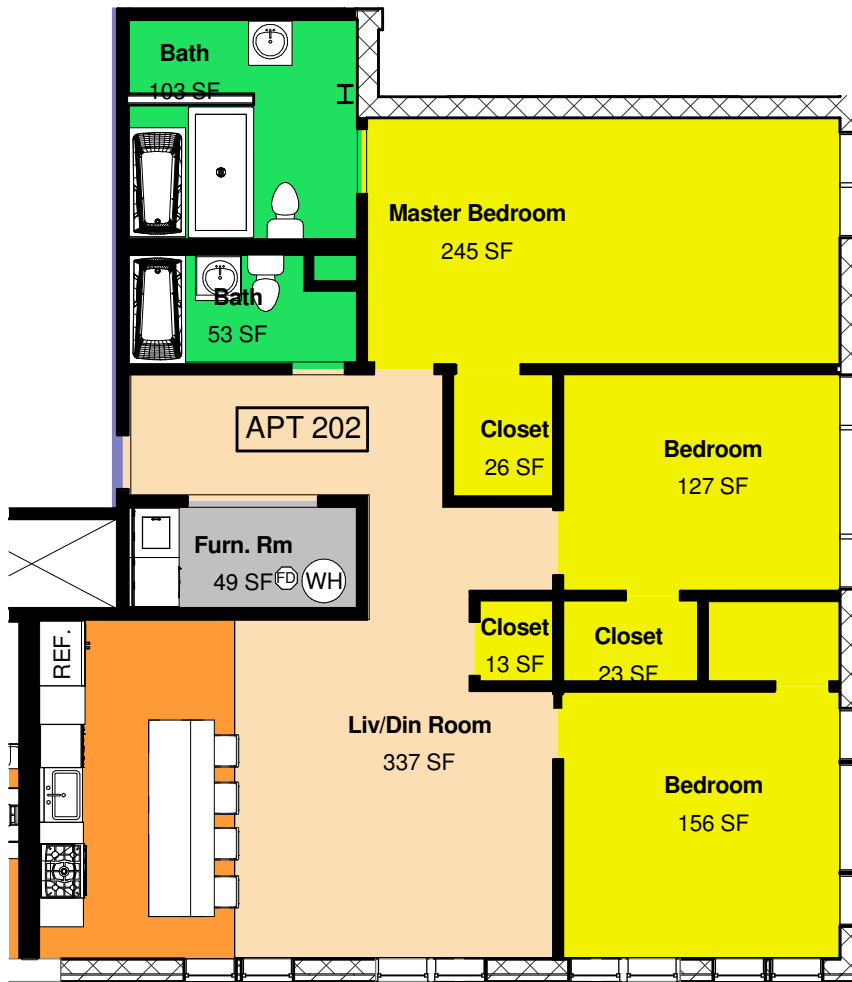
① Enlarged Proposed 2nd Floor Apt 202 - 1244 SF 1/8" = 1'-0"
