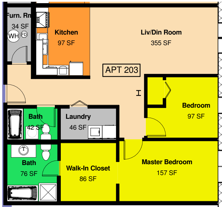
① Enlarged Proposed 2nd Floor Apt 203 - 1056 SF 1/8" = 1'-0"
