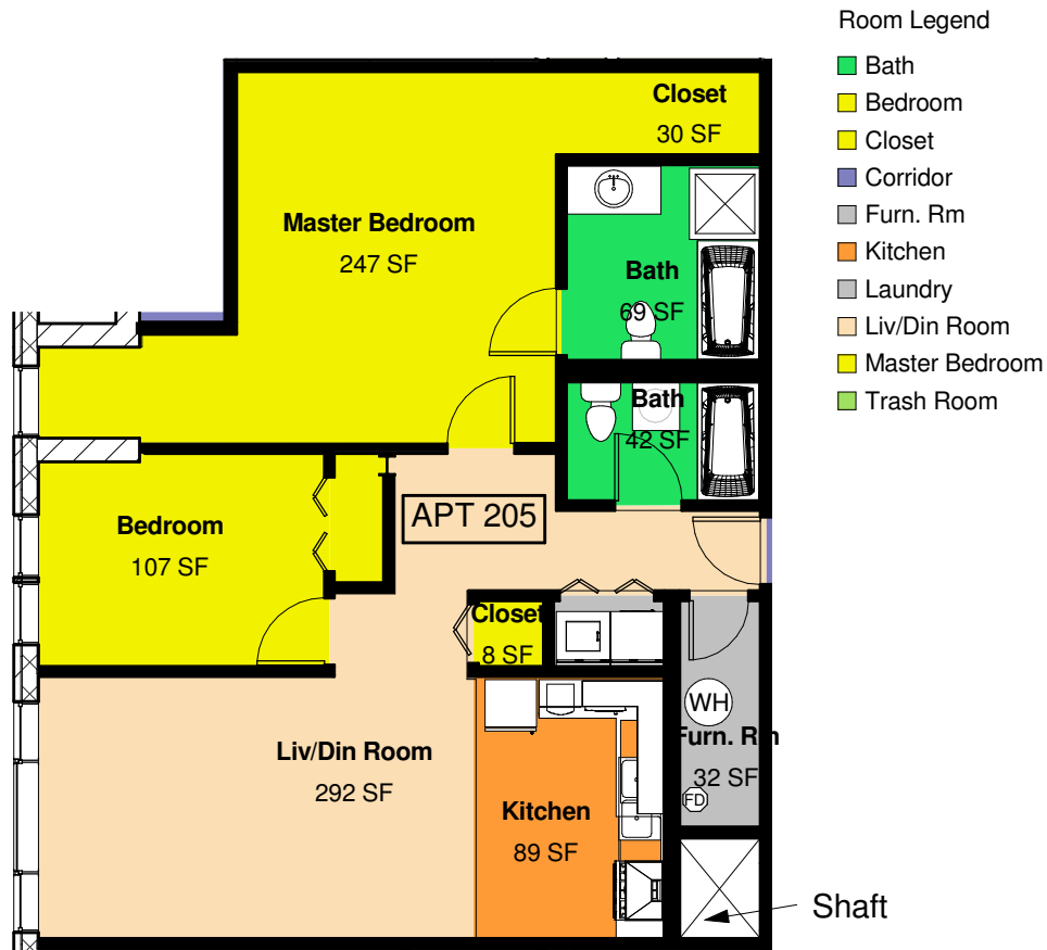
① Enlarged Proposed 2nd Floor Apt 205 - 1078 SF 1/8" = 1'-0"
