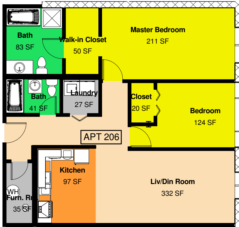
① Enlarged Proposed 2nd Floor Apt 206 - 1012 SF 1/8" = 1'-0"
